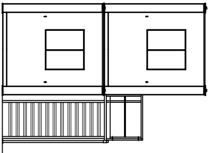
LEFT ELEVATION
