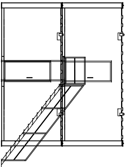
FRONT ELEVATION
